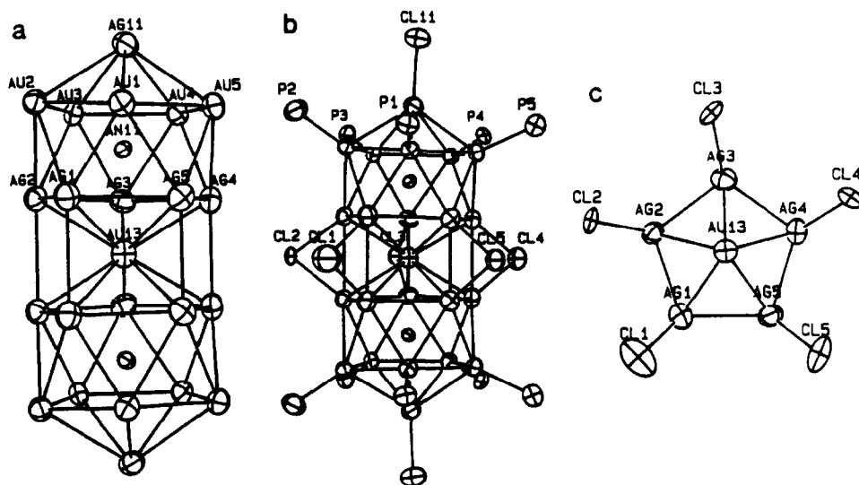
Fig. 6. Molecular architecture of [(\text{Ph}_3\text{P})_{10}\text{Au}_{12}\text{Ag}_{12}\text{NiCl}_7]^+ , as the \text{SbF}_6^- salt: (a) the metal core, \text{Au}_{12}\text{Ag}_{12}\text{Ni} ; (b) the metal-ligand framework, \text{P}_{10}\text{Au}_{12}\text{Ag}_{12}\text{NiCl}_7 ; (c) projection of the two silver pentagons onto the five doubly bridging chloride ligands CL1–CL5. Atoms AN11 and AN11' (centers of icosahedra) represent an equal admixture of Au and Ni owing to the crystallographically imposed mirror ( C_s -m) symmetry.
