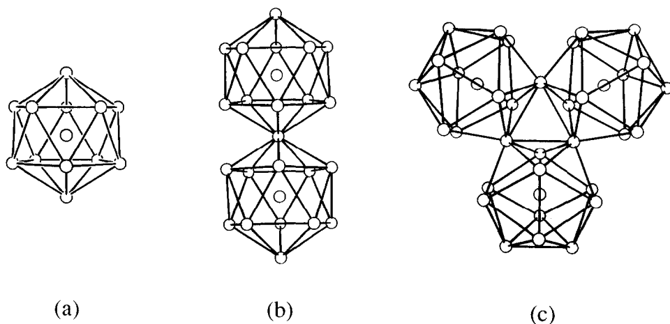
Fig. 2. The first three members of vertex-sharing polyicosahedral supraclusters: (a) icosahedron; (b) biicosahedra; (c) triicosahedra.
