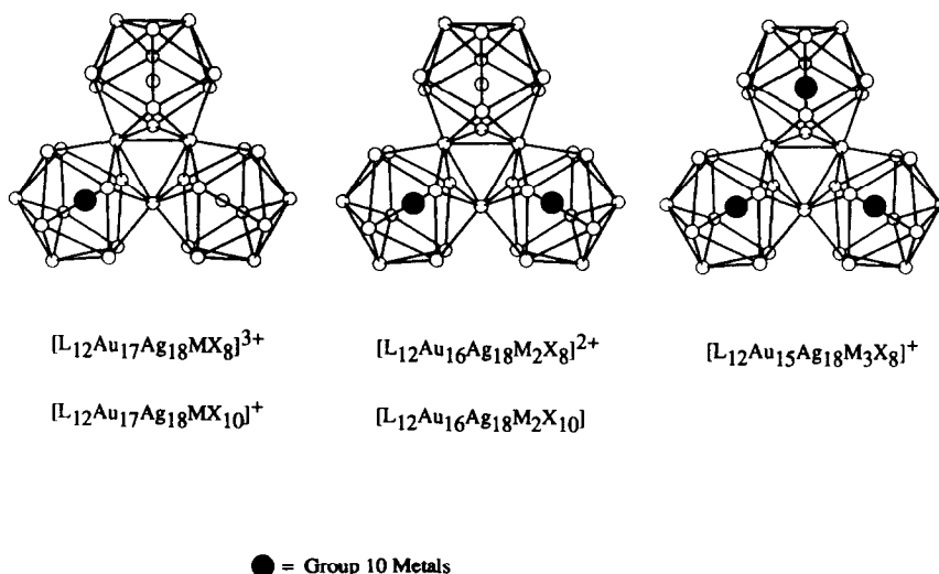
Fig. 7. endo icosahedral chemistry: trimetallic (Au–Ag–M) triicosahedral clusters with one, two, and three group 10 (M = Pt, Pd, Ni) metals at the center(s) of icosahedra.
